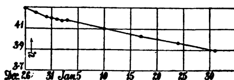
FIG. 33.—Chart showing loss of standard volumes of gas in diver in lapse of days. Diffusion of air through K_2SO_4 solution.
